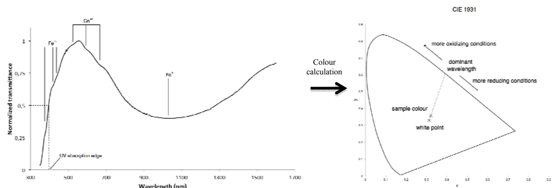
Figure 1 – The left graph shows the optical absorption spectrum of a glass fragment. The main colouring agent is iron, but the presence of cobalt impurities is detected. The UV absorption edge is also pointed. The right graph shows how to determine the dominant wavelength in CIE1931 horseshoe system.
