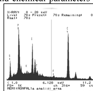
Fig. 2 – SEM+EDS analysis of the surface of the Adriano's coin
